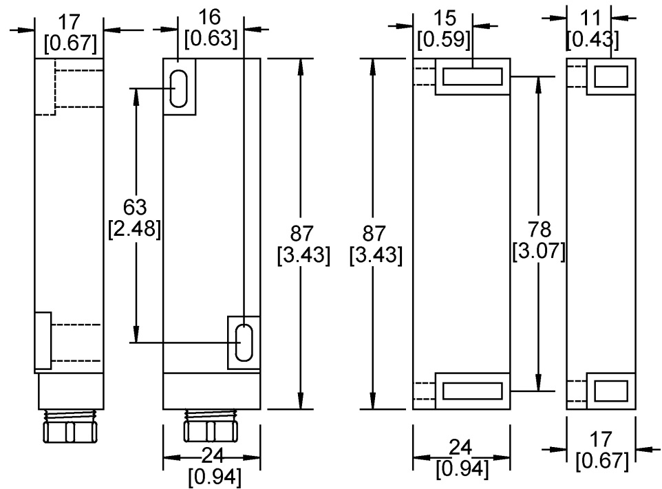
SWITCH
